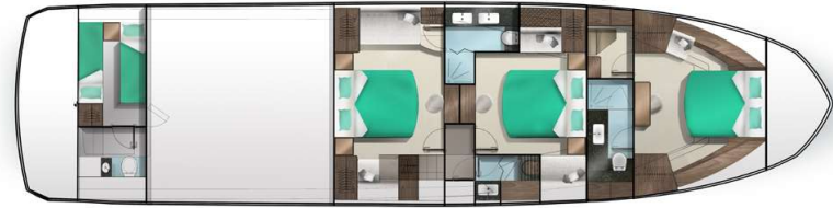
Three Master cabin layout ver. 1
